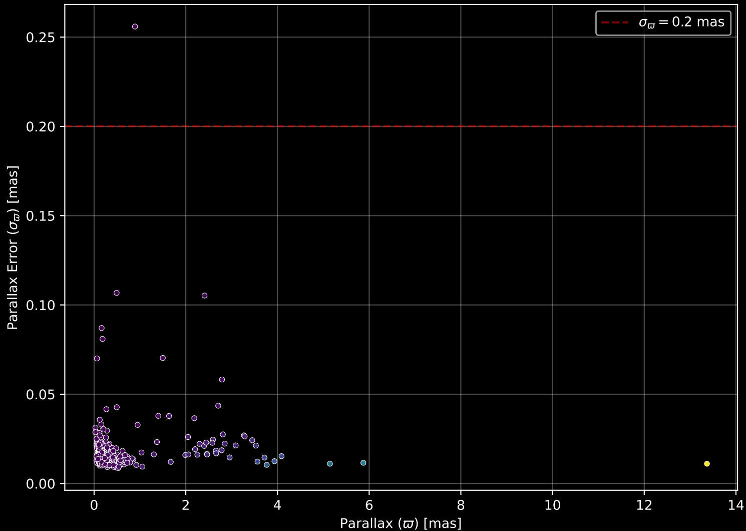
APOGEE DR17 Field: [240-08] Parallax Quality (n= 416)
