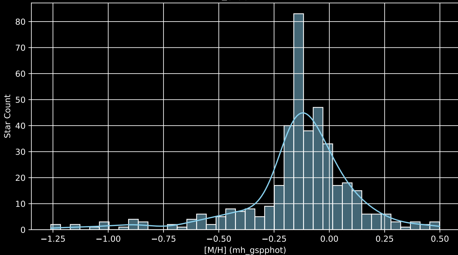
APOGEE DR17 Field: [240-08 [M/H] (mh_gspphot) (n= 411)
