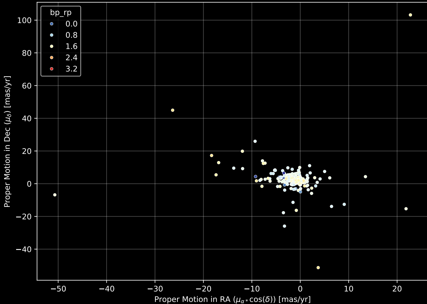
APOGEE DR17 Field: [240-08] Proper Motion Diagram (n= 416)
