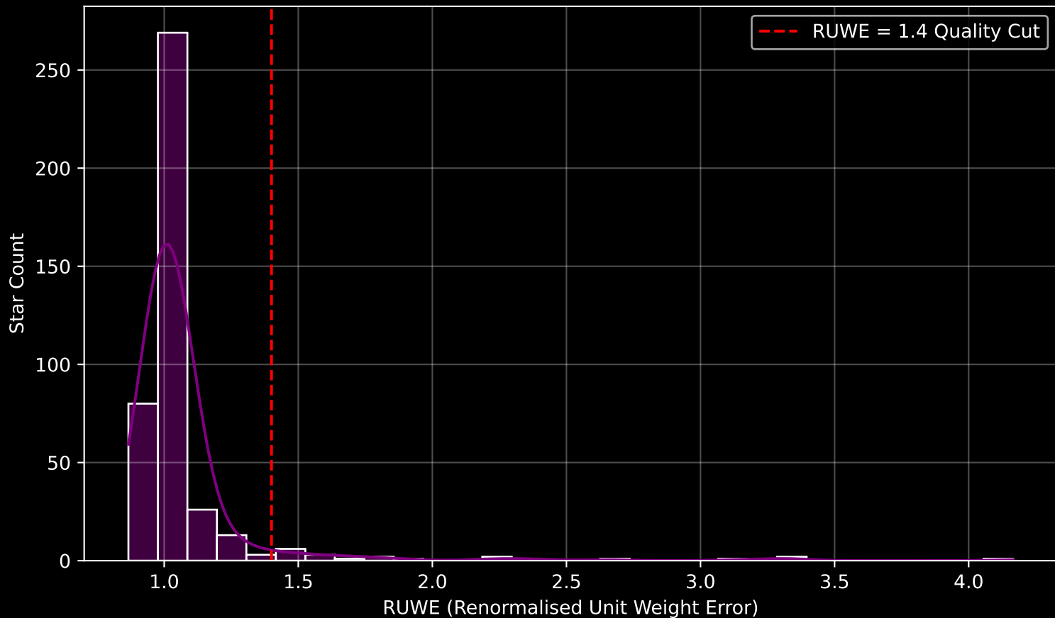
GAPOGEE DR17 Field [240-08] RUWE Distribution (n= 412)
