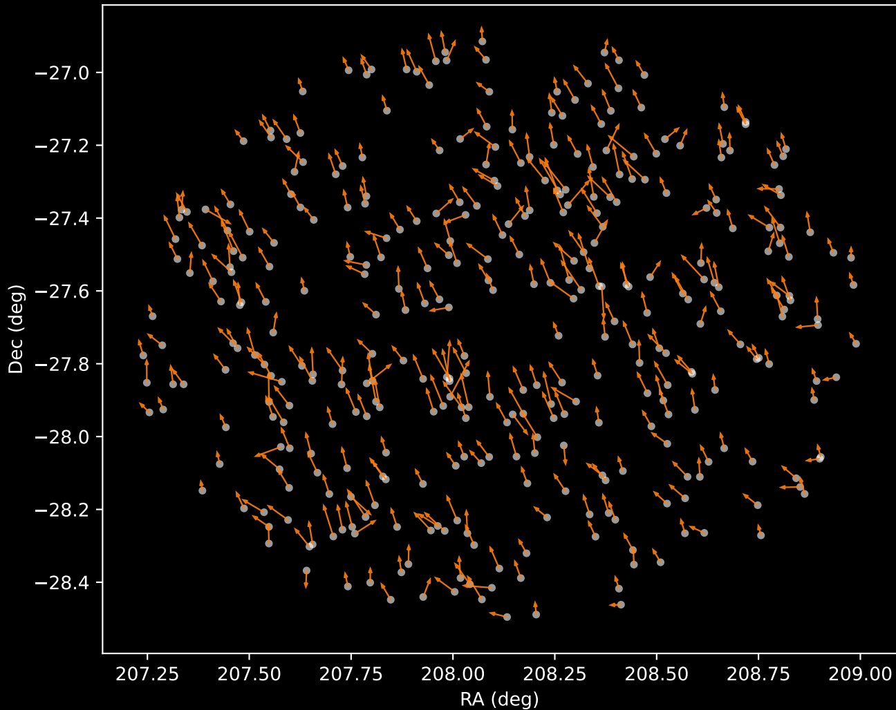
APOGEE DR17 Cluster 2 Proper Motion Vectors (n=357)
